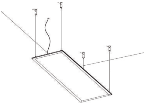
4. Pendent installation
